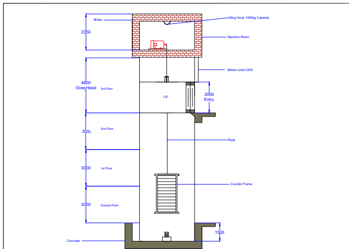
Machine Room (Traction)
